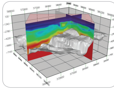
Input model for ray tracing
