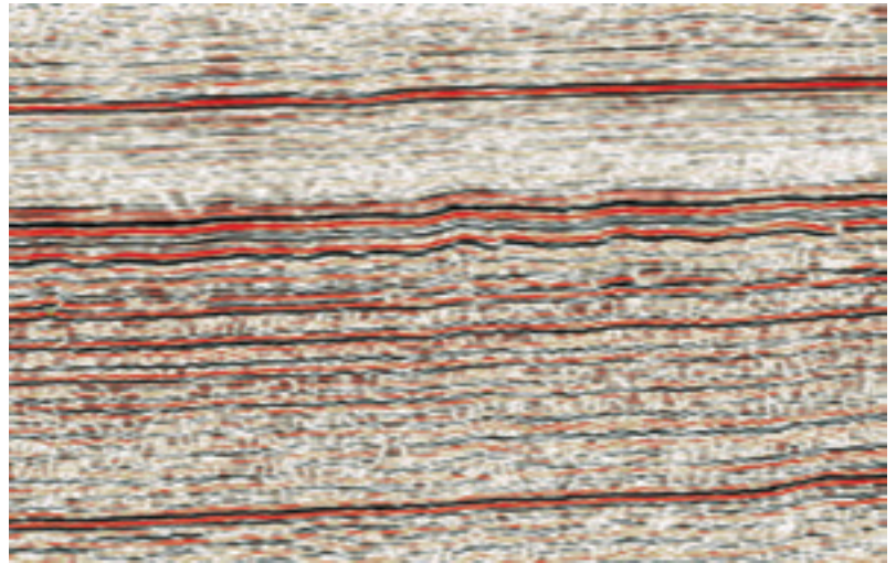
P-wave data from ION's Lakeview SCAN
